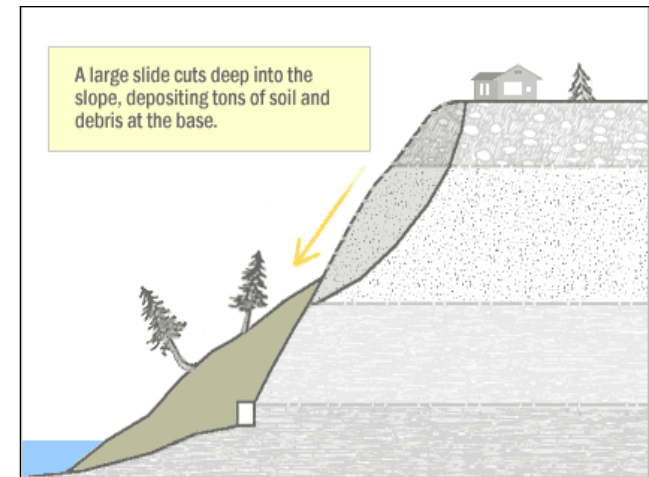
FIGURE 10-4. LARGE SLIDE
