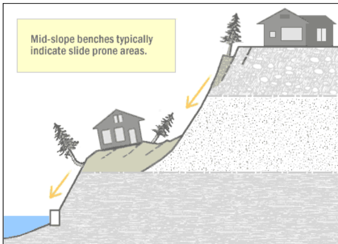
FIGURE 10-3. BENCH SLIDE
