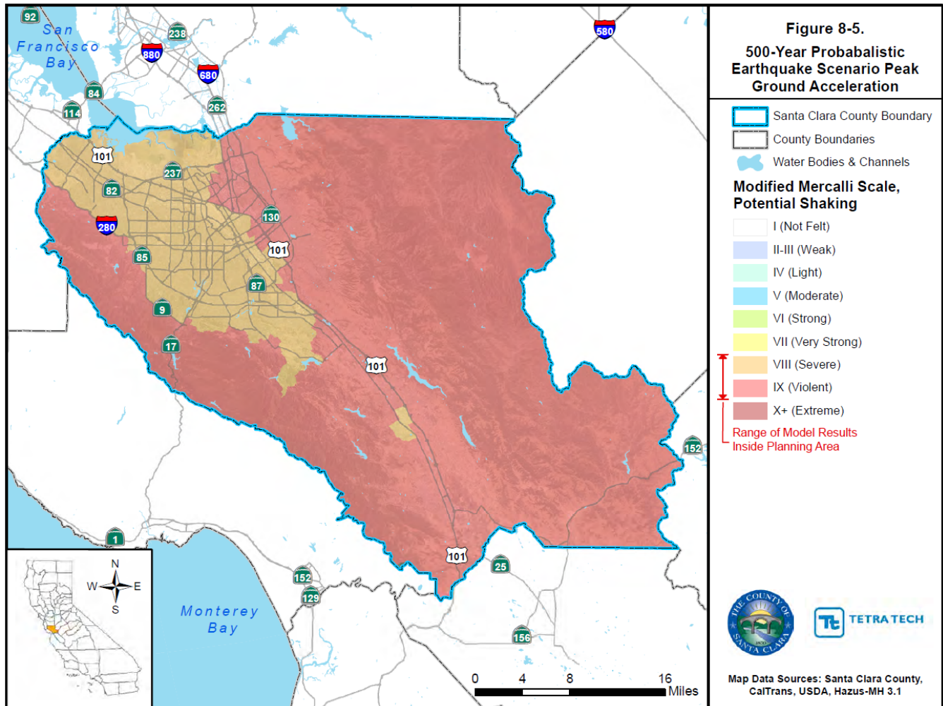
Figure Shake Maps
