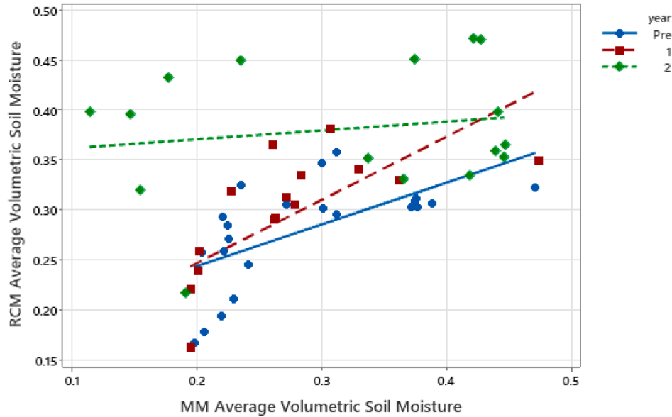
Figure 16. Regression plots by year for the average weekly volumetric soil moisture for Rock Creek and Marian Meadows 2020-2022. Year is the sequence of water years since restoration Year = 2 is the water year following the Dixie Fire (2022 WY) and is statistically different from pre-restoration year, while Year =1 is not statistically different; p values <0.001 and 0.45 respectively (Table 9). In contrast to Marian and Control Meadows there was not a statistical difference in the slopes of the regression lines, even though the fitted lines are illustrated at different slopes.
