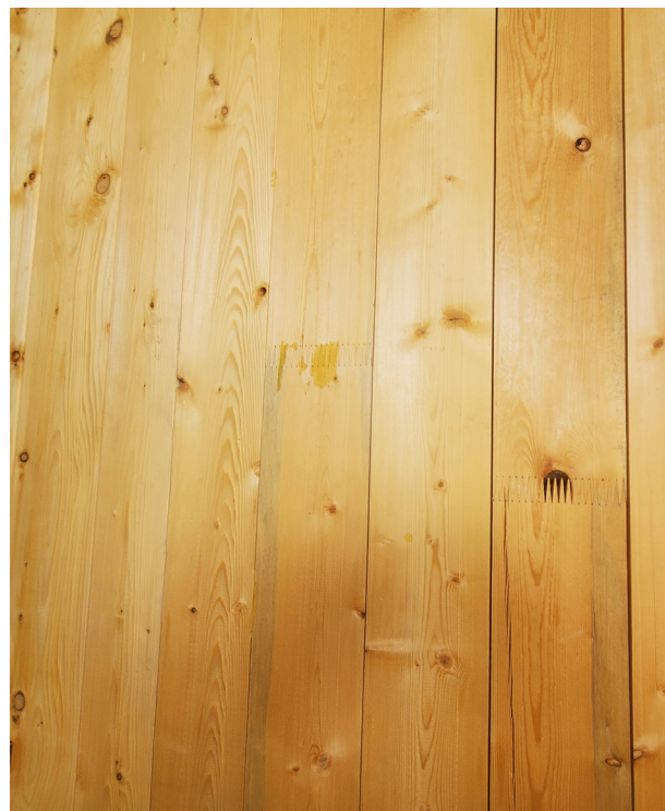
A CLT wall with finger joints
