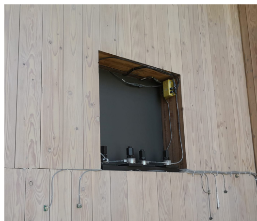
Moisture sensors at Oregon State University's Peavy Hall are used to detect moisture content of the mass timber panels
