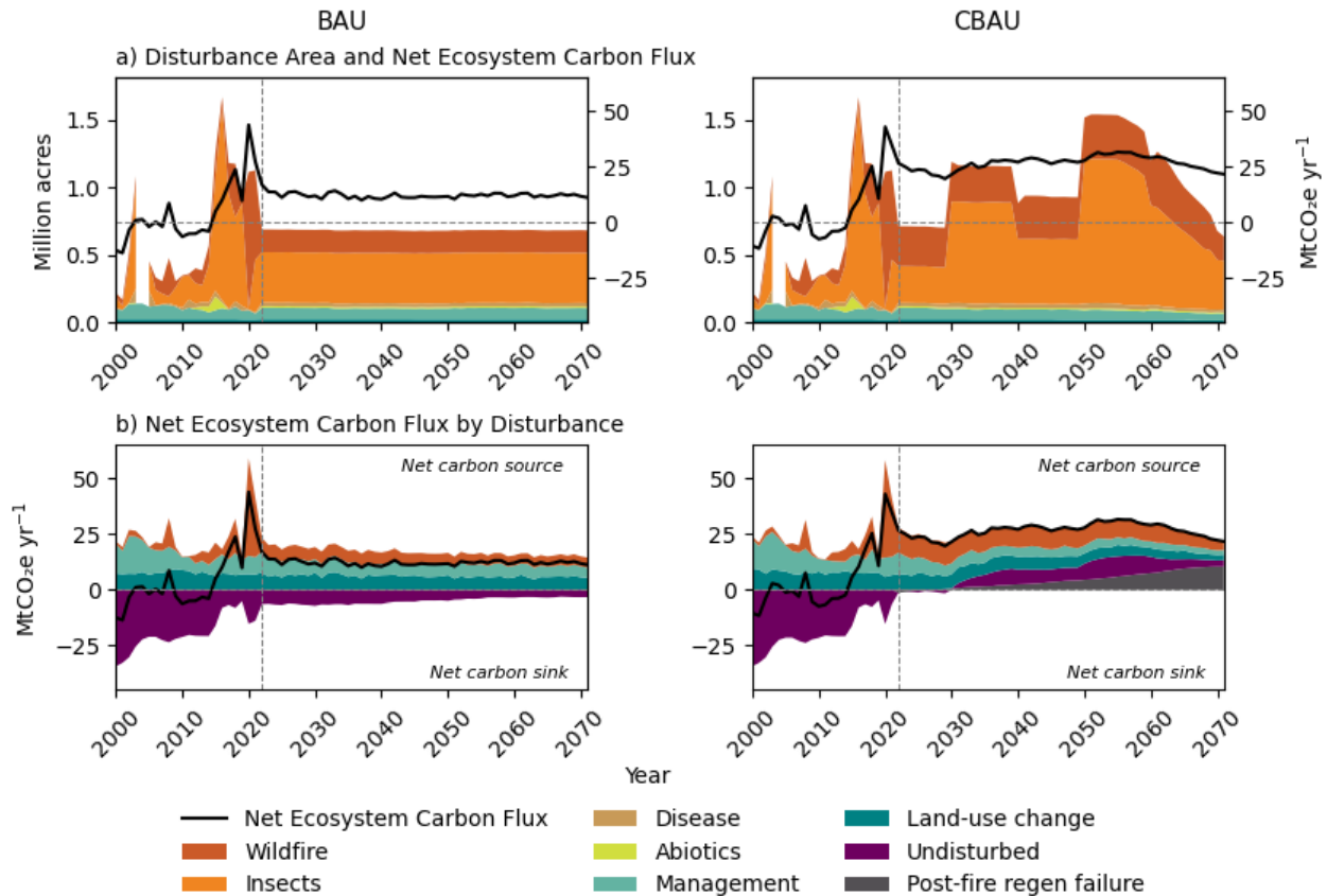
Figure 6. BAU and CBAU scenario results showing a) disturbance area (million acres) by disturbance type and net ecosystem carbon flux (MtCO 2e yr -1 ), and b) annual net ecosystem carbon flux (MtCO 2e yr -1 ) by disturbance type from 2000–2071. Net ecosystem carbon flux refers to the net yearly sequestration of carbon by forests across all 14 ecosystem carbon pools, after accounting for decomposition, natural disturbance emissions, and wood product transfers. In Panel b), negative numbers for net ecosystem carbon flux represent a net carbon sink and positive numbers represent a net carbon source.
