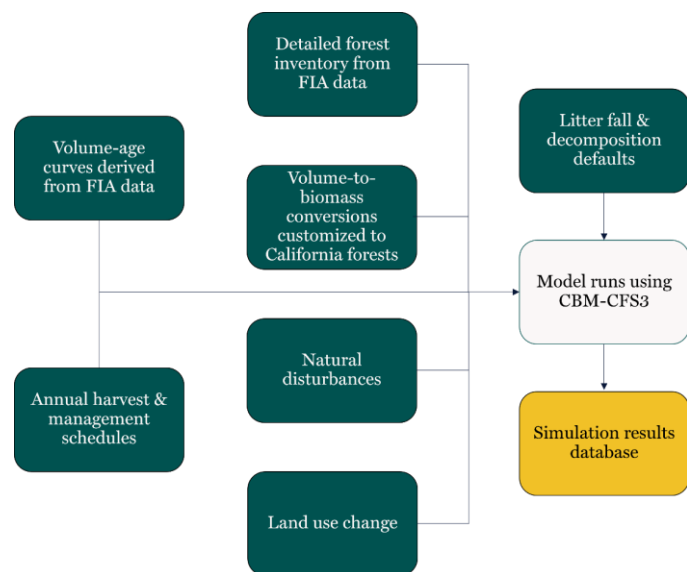
Figure 2. Modeling inputs and process for CBM-CFS3. Adapted from Kull et al. 2019.
