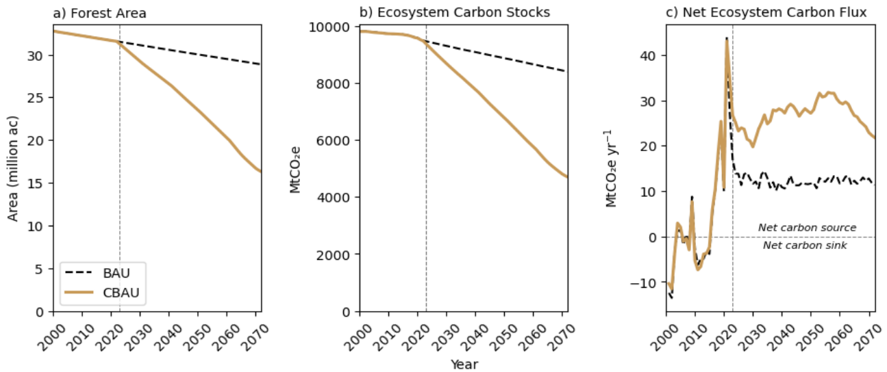
Figure 5. BAU and CBAU scenario results showing a) total forest area (million acres), b) ecosystem carbon stocks (MtCO 2e ), and c) annual net ecosystem carbon flux (MtCO 2e yr -1 ) from 2000–2071. Net ecosystem carbon flux refers to the net yearly sequestration of carbon by forests across all 14 ecosystem carbon pools, after accounting for decomposition, natural disturbance emissions, and wood product transfers. In Panel c), negative numbers for net ecosystem carbon flux represent a net carbon sink and positive numbers represent a net carbon source.
