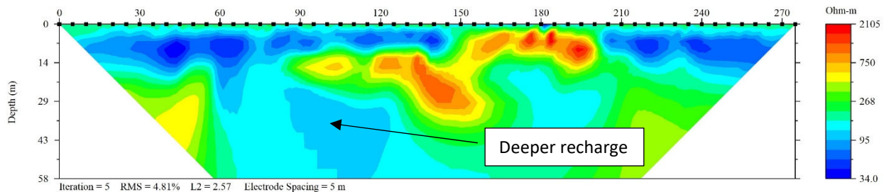
Figure 14. Rock Creek Deep Electrical Resistivity Profile. This profile trends from the road bisecting Rock Creek Meadow toward instrument and vegetation transect site 1 (Figure 3). The right side of the image (horizontal position of 275 meters) is located at (40.3307^\circ, -121.0873^\circ) , with a heading of 40^\circ . The electrode spacing is 5 meters. Data was collected with a dipole-dipole-gradient pattern.
