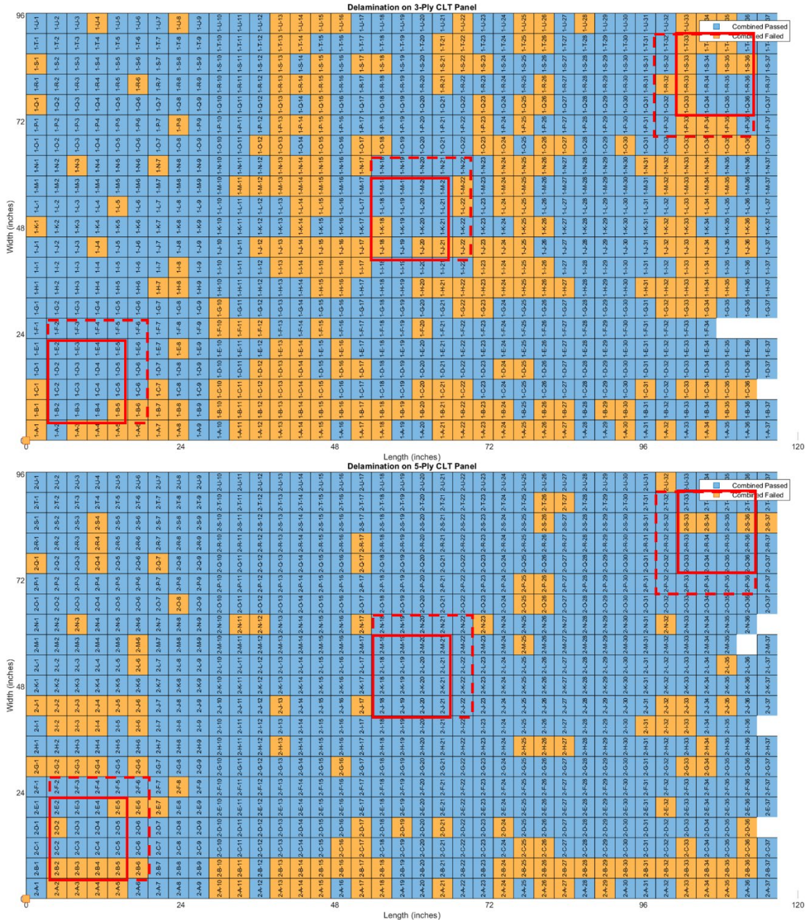
Figure 11. Distribution of specimens failing PRG320-2019 delamination criterion in 3-ply (top) and 5-ply (bottom) MF panels with possible sampling areas marked as solid and dashed red rectangles.
