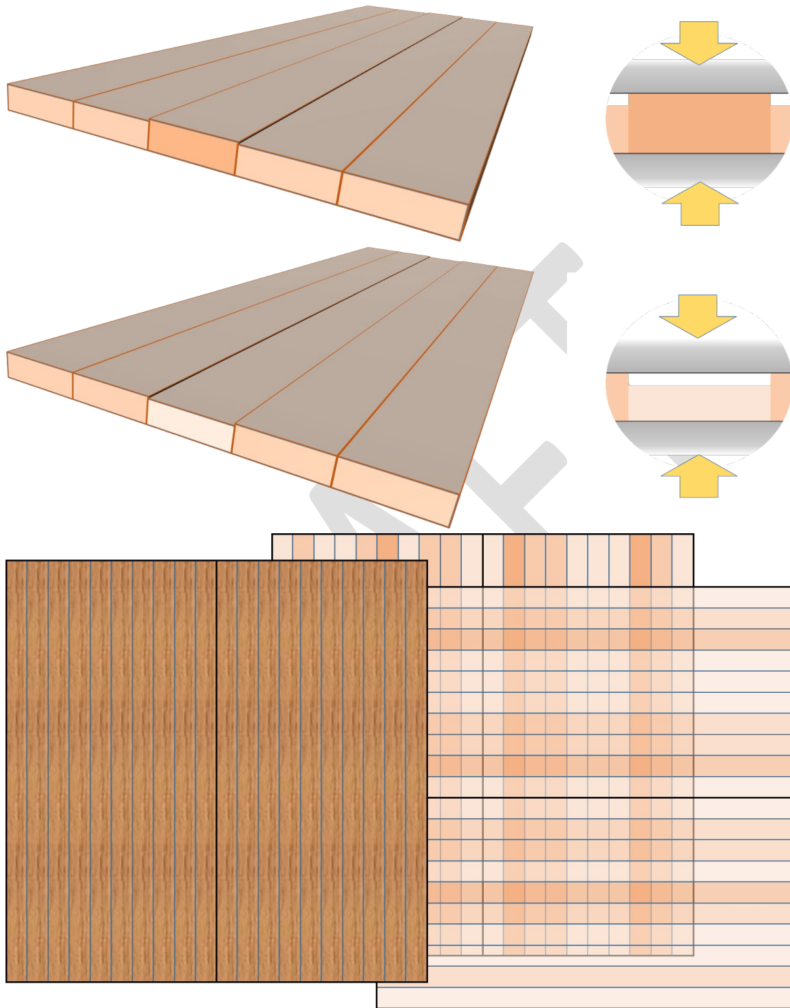
Figure 14. Schematic diagram illustrating propagation of thickness variation along the lamination within one layer, and a potential for bridging when layers with variable lamination thicknesses are cross laminated.
