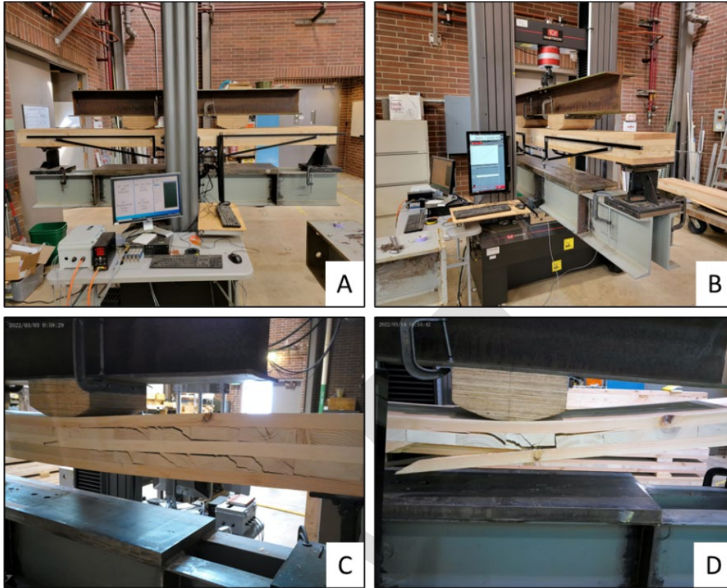
Figure 6: (A&B) Long-Span Flexure Test setup, (C) Typical 5-ply sample failure (Shear failure), (D) Typical 3-ply sample failure (Tension failure)
