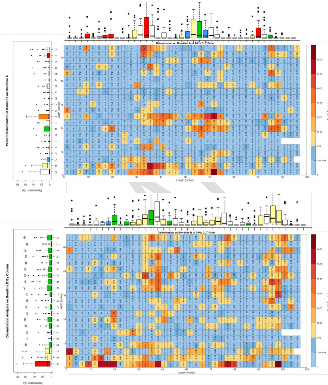
Figure 15. Distribution of frequency of delaminations within individual bond planes in 3-ply MF panels within horizontal and vertical strips. Alignment along individual laminations may be an indication of an effect of lamination thickness variation
