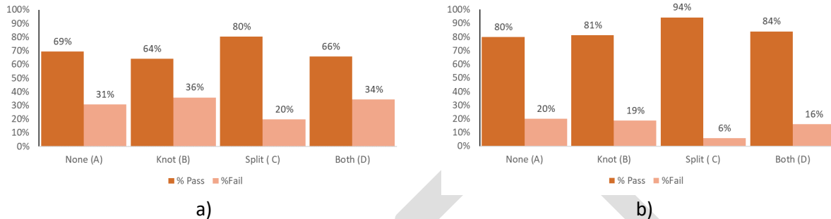
Figure 13. Comparison of proportions of specimens passing and failing the PRG320-2019 delamination tests in 3-ply (a) and 5-ply (b) MF panels by categories: clear specimens (A), specimens with knots touching a bond plane (B), specimens with inter-lamination gaps (C) and with both, knots and gaps (D). (Based on n=775 in both panels).
