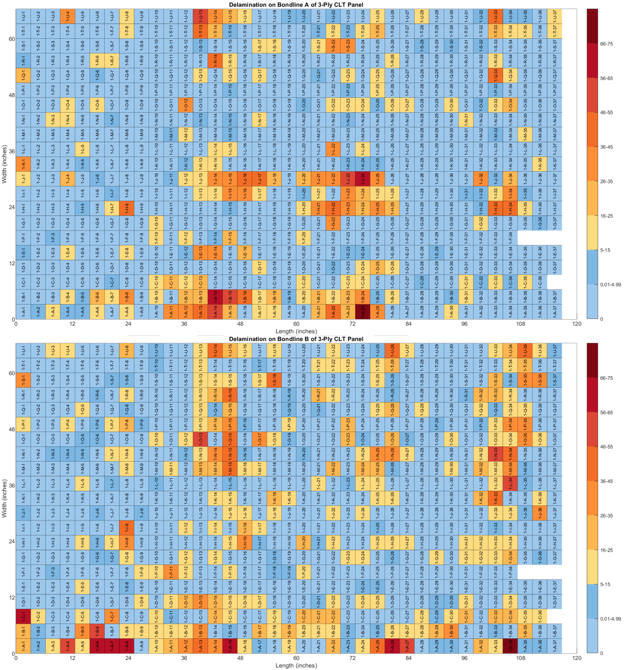
Figure 10. Color coded Delamination map for two bond planes in 3-ply MF panel. Color scale reflects the percent of delamination in each block measured after PRG320-2019 PRG delamination test (shades of blue show acceptable level of delamination or pass).
