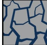
Drought SECTION 4.5.4
