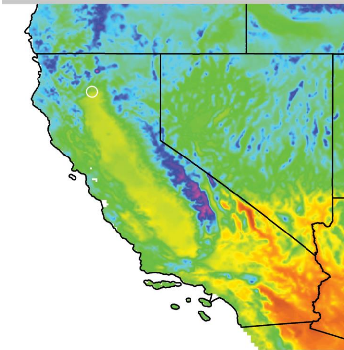
RCP 4.5 YEAR 2100
