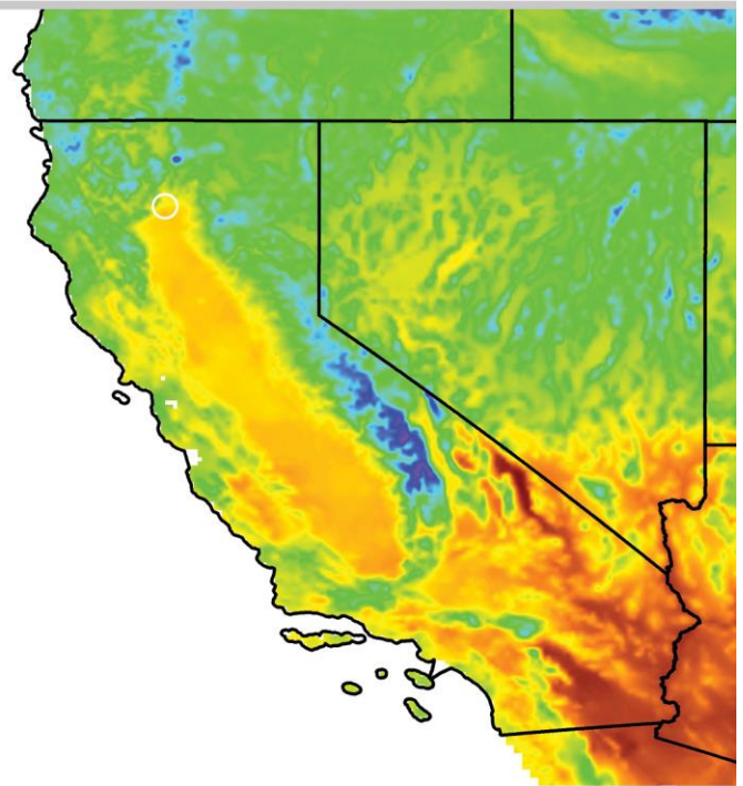
RCP 8.5 YEAR 2100
